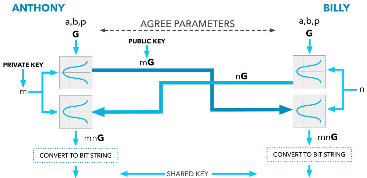
Figure 3: ECDH
