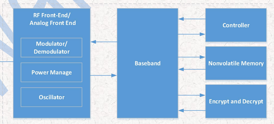
Figure 2.6 The project's reader IC solution block diagram
